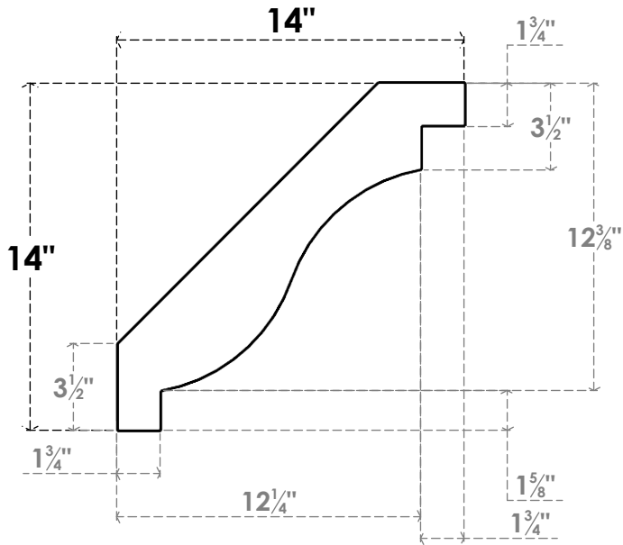
SIDE PROFILE
